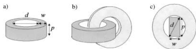
Figure 2. a) Labeling system for dimensions of a solid circular ring, d = inner diameter, w = edge width, p = depth; b) two such rings interpenetrating; c) limiting situation for the two interpenetrating rings, revealing the geometric constraint d^2 \geq w^2 + p^2 . [24]
